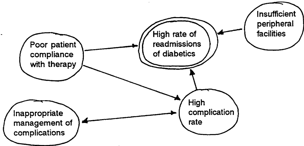
Figure 4.2. Initial problem diagram - diabetes.
