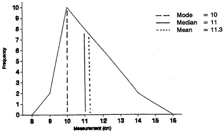
Figure 22.7. Mean, median, and mode in a distribution curve.
