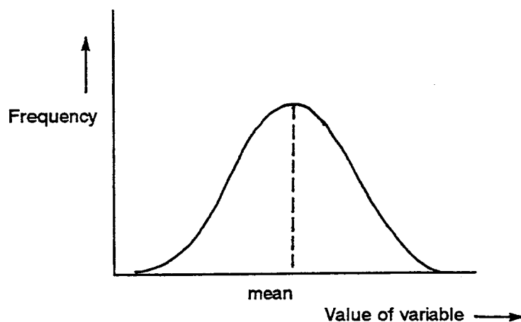
Figure 25.1. Normal distribution curve.
