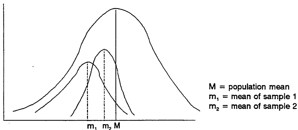
Figure 25.4. A frequency distribution curve and two sample curves for a variable that is normally distributed.
