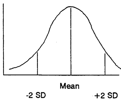
Figure 25.3. A normally distributed variable.
